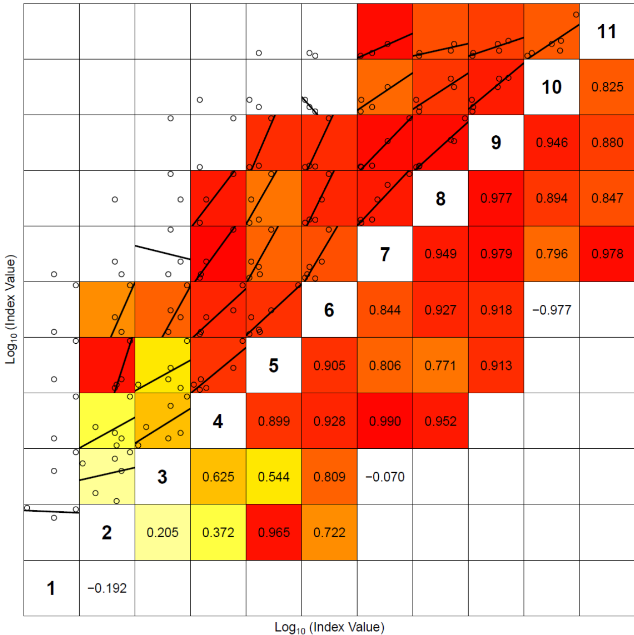
Figure 19. Preliminary results. Internal consistency for Norwegian spring-spawning herring within the IESSNS 2022. The upper left part of the plots shows the relationship between log index-at-age within a cohort. Linear regression line shows the best fit to the log-transformed indices. The lower-right part of the plots shows the correlation coefficient ( r ) for the two ages plotted in that panel. The background colour of each panel is determined by the r value, where red equates to r =1 and white to r <0.
