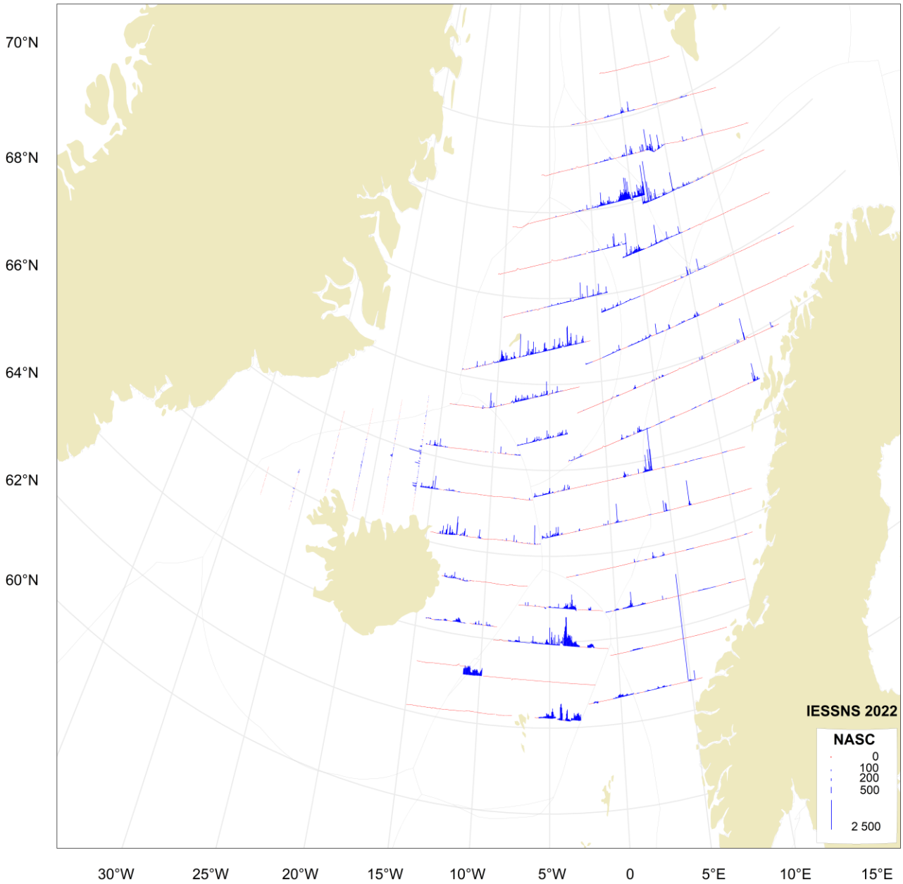
Figure 17b. Preliminary results. The s_A /Nautical Area Scattering Coefficient (NASC) values of Norwegian spring-spawning herring along the cruise tracks in 2022, presented as bar plot.
