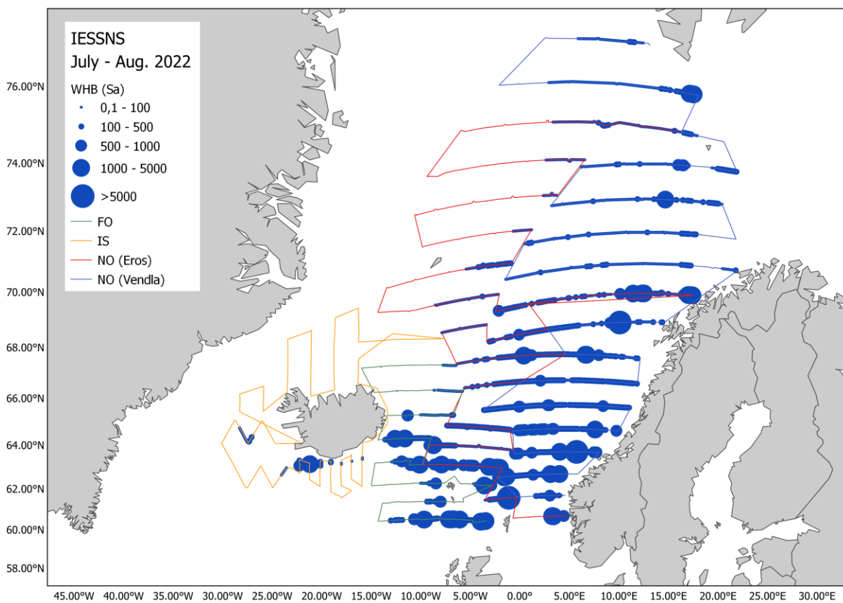
Figure 20a. Preliminary results for the s_A /Nautical Area Scattering Coefficient (NASC) values of blue whiting along the cruise tracks in IESSNS 2022.
