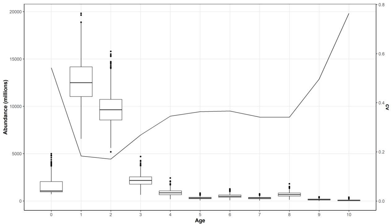
Figure 21. Preliminary results of number by age with uncertainty for blue whiting during IESSNS 2022. Boxplot of abundance and relative standard error (CV) obtained by bootstrapping with 1000 replicates using the StoX software.
